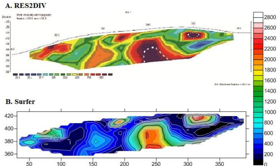
Figure 2. 2D Geoelectric Interpretation of dipole-dipole results; A. Vertical interpretation of mapping using the Res2DIV software; B. Vertical interpretation of mapping using Surfer software
